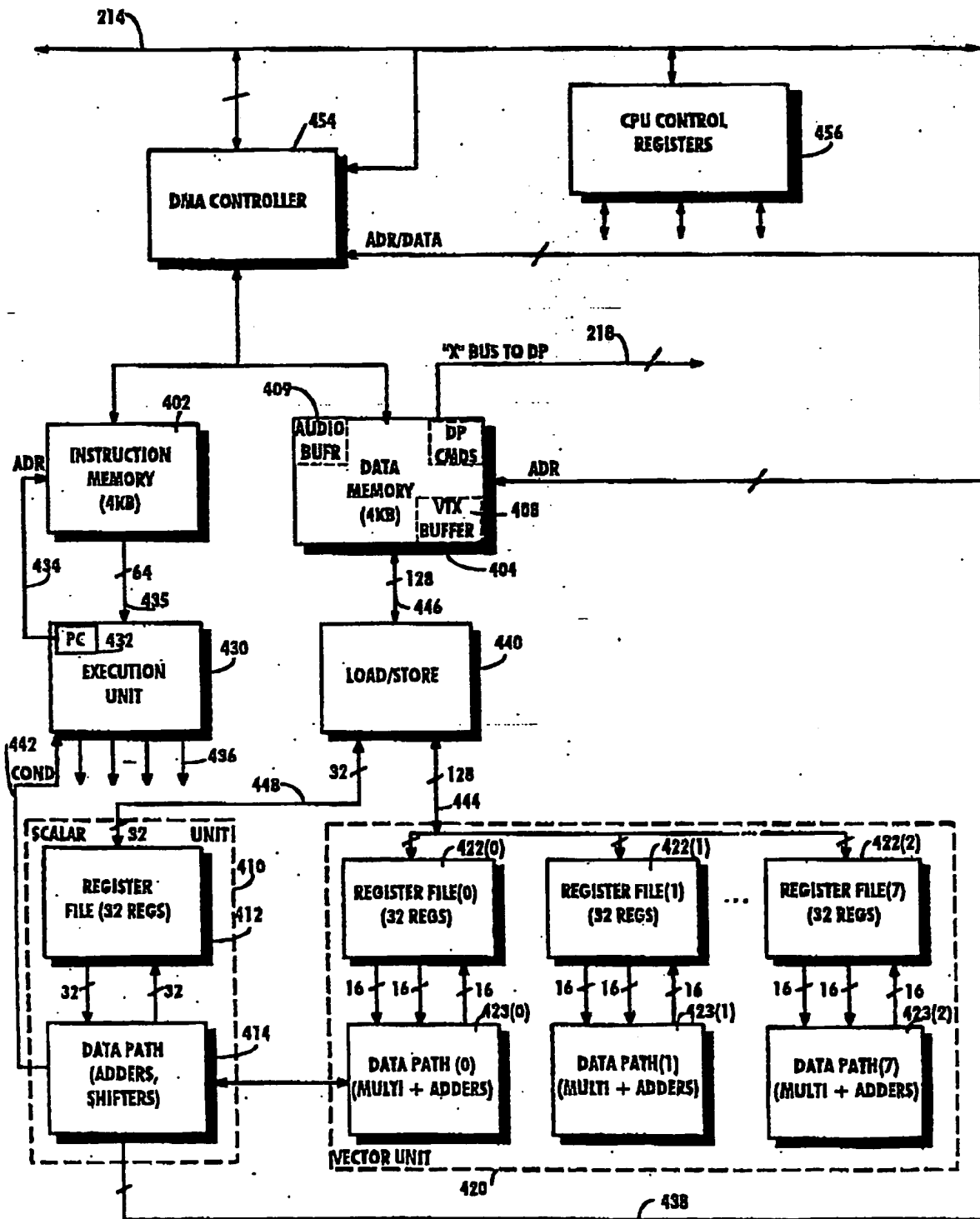
Fig. 7 SIGNAL PROCESSOR 400
